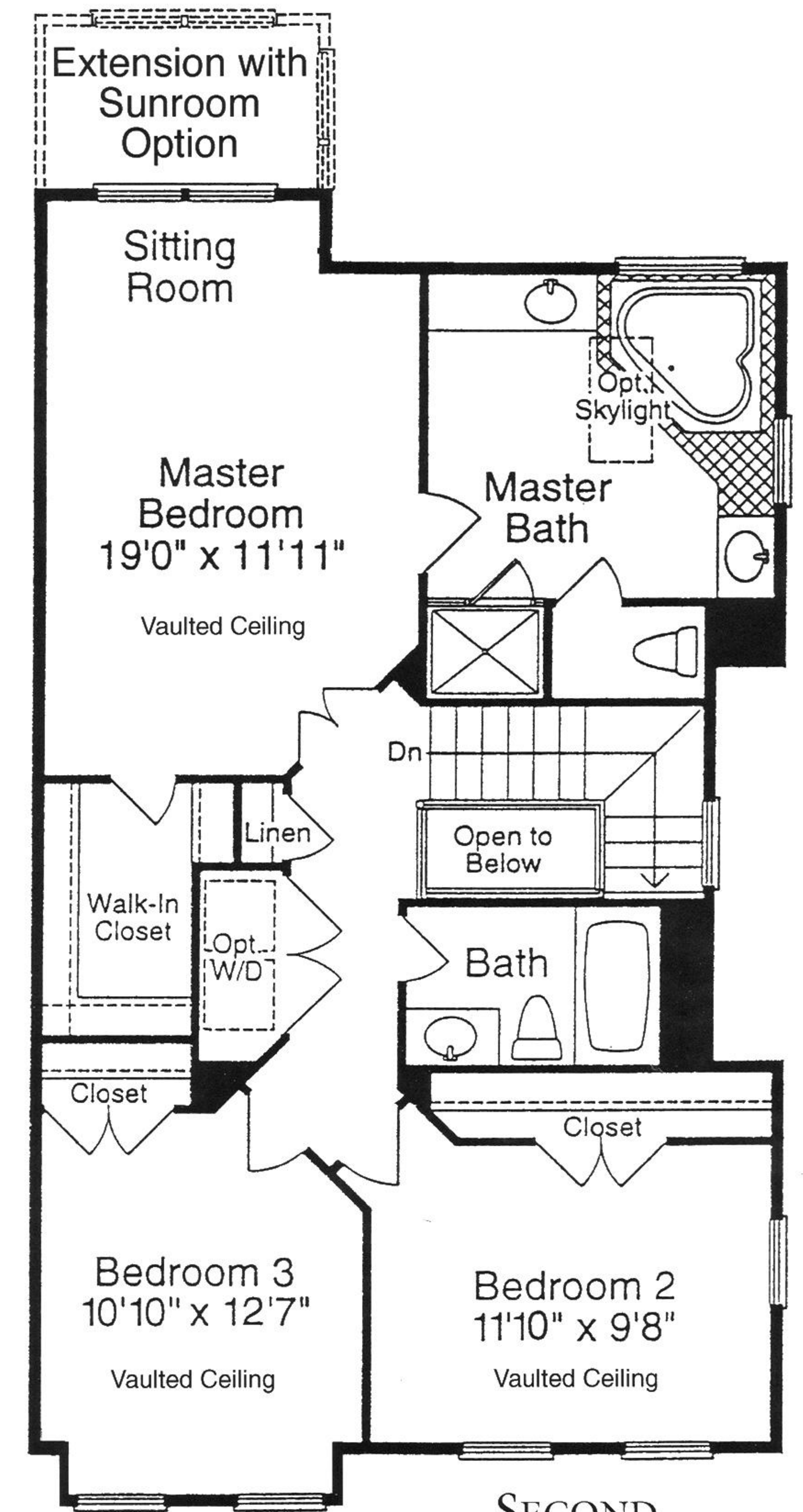
SECOND FLOOR PLAN
